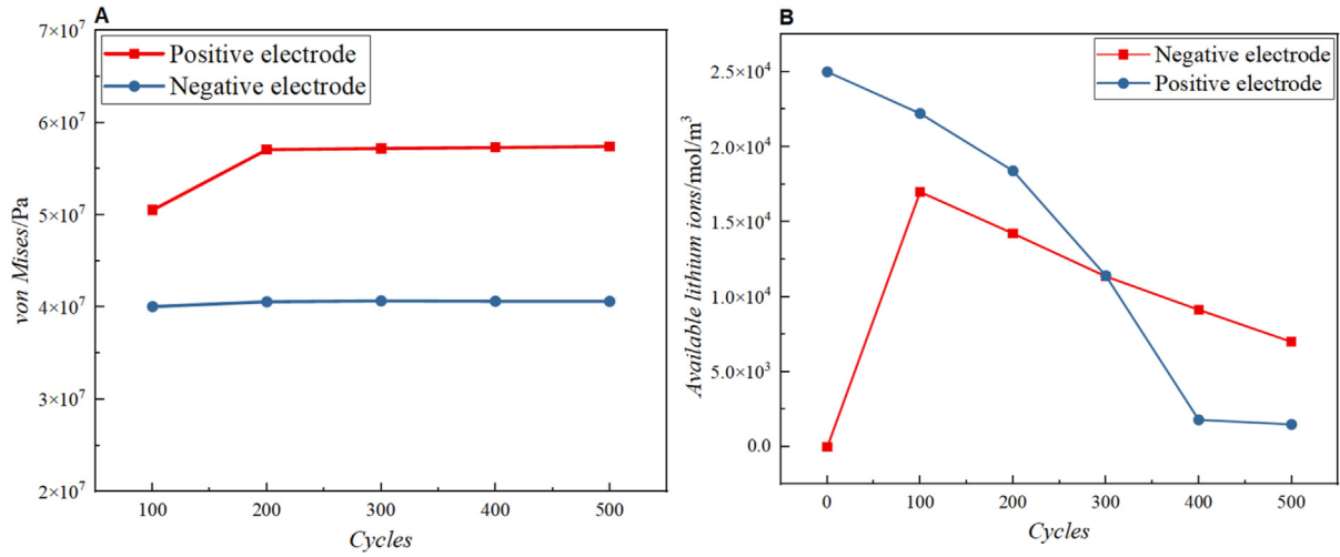
Fig. 13. The von Mises stresses (A) and available lithium ions concentrations (B) of positive and negative electrodes upon different cycles under 3C rate.
