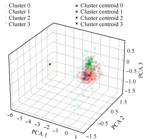
Fig. 10 Results obtained using GMM clustering and centroids used for the anomaly detection task.
