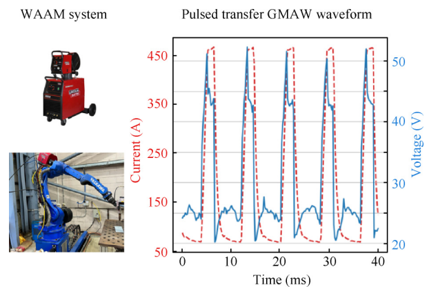
Fig. 3 Experimental setup and waveform welding process employed. Traditional Pulse welding consists of a peak and background current to deposit a molten droplet after each pulse. The waveform, described by parameters like Pulse ramp, tailout and background current, is developed by a welding supplier and allows to deposit of a droplet with a fixed frequency depending on wire material and diameter.
