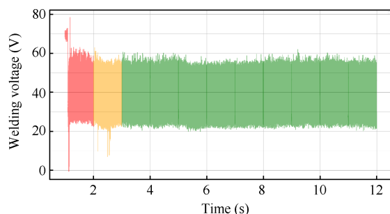
Fig. 16 Results of the proposed monitoring methodology based on clustering and unsupervised machine learning in detecting the WAAM states during the deposition and in identifying anomalies.
