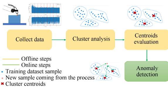
Fig. 8 Proposed methodology for anomaly detection based on clustering analysis and centroid-distance methods.
