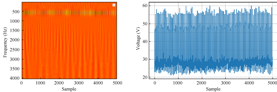
Fig. 11 Spectrogram and time series welding voltage signal of cluster 0 medoid.
