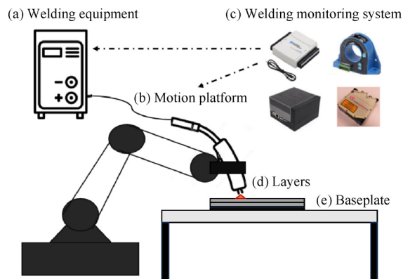
Fig. 1 Wire Arc Additive Manufacturing utilizes an electric arc to selectively melt a wire feedstock, enabling a layer-by-layer deposition to create near-net-shape components. A Welding Monitoring System can be used to collect data from the process and take action based on the data.
