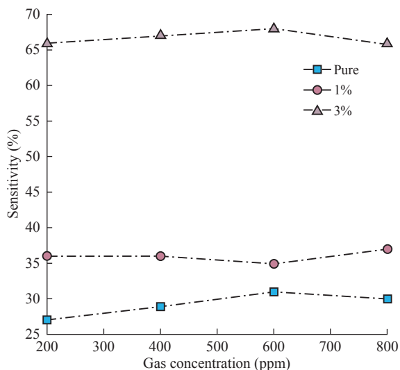
Fig. 8 Percentage sensitivity change of \text{Co}_3\text{O}_4 : Mn films for changed concentrations of \text{NO}_2 gas at a working temperature of 150^\circ\text{C} .
