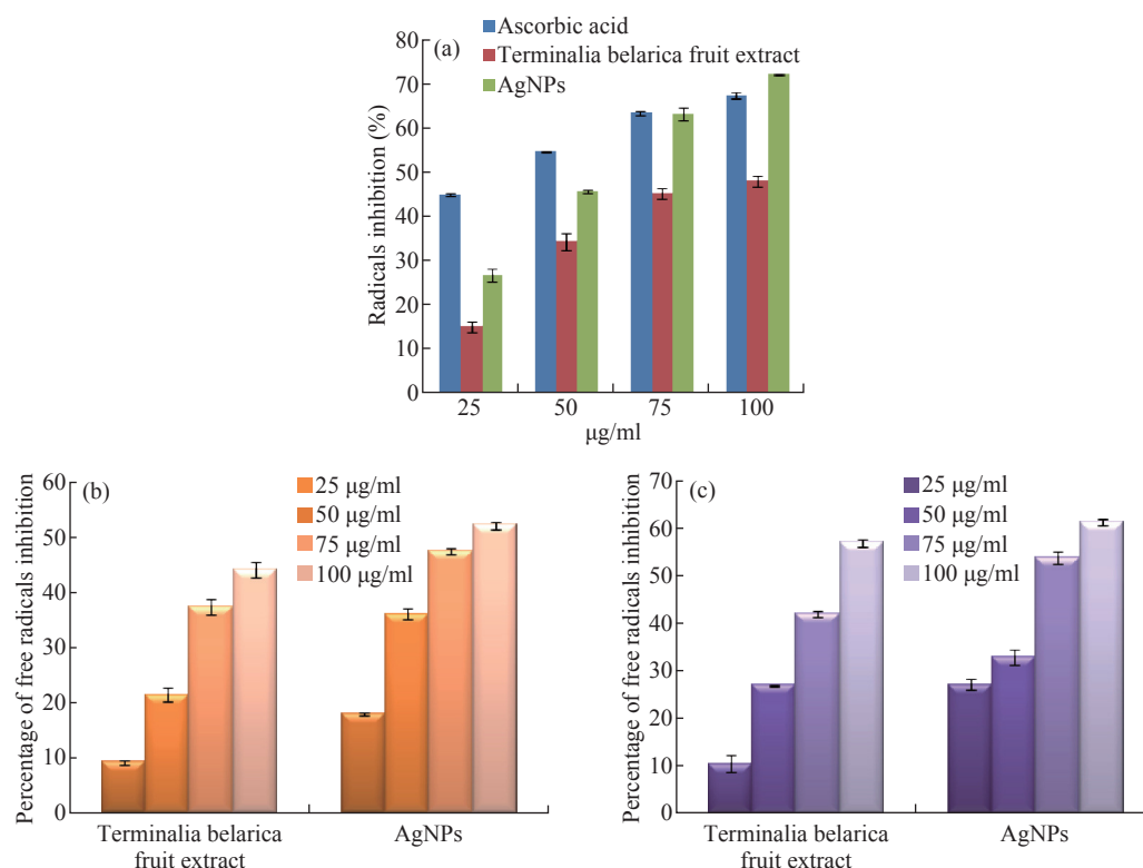
Fig. 11 (a) Free radical scavenging activity of biofabricated Tb -AgNPs by DPPH method; (b) Free radical scavenging activity of biofabricated Tb -AgNPs by H_2O_2 method; (c) Free radical scavenging activity of biofabricated Tb -AgNPs by NO method.
