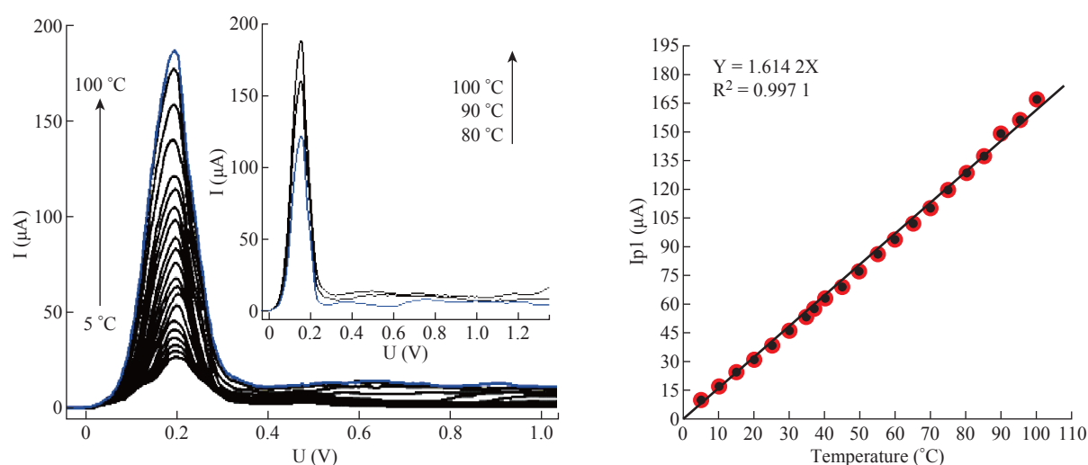
Fig. 12 Polarographic waves of 5-FU drug (10 \mu M) at different temperatures in aqueous solutions of potassium phosphate buffer at pH = 7.0 and under optimum conditions.
