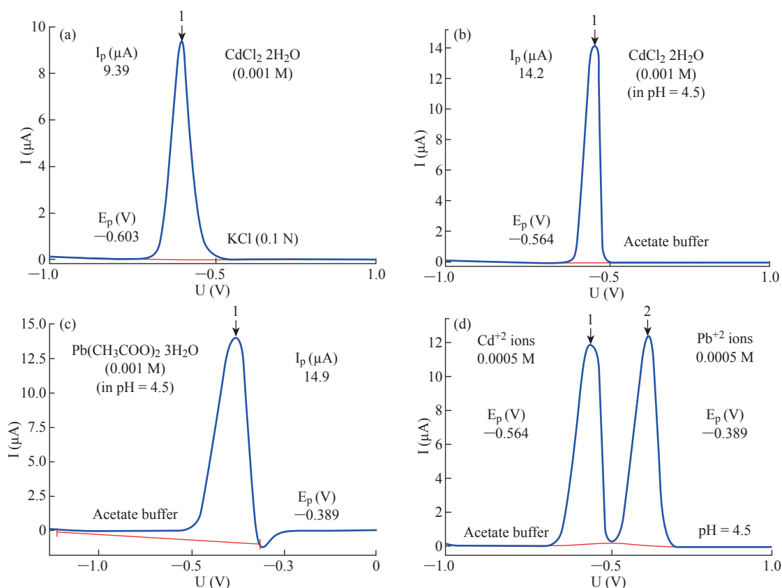
Fig. 3 Standardization of polarographic analyzer, 797 VAcomputrace. (a) 0.001 M \text{CdCl}_2 \cdot 2\text{H}_2\text{O} in 0.1 M KCl; (b) 0.001 M \text{CdCl}_2 \cdot 2\text{H}_2\text{O} in acetate buffer at pH = 4.5; (c) 0.001 M \text{Pb}(\text{CH}_3\text{COO})_2 \cdot 3\text{H}_2\text{O} in acetate buffer at pH = 4.5; and (d) 0.0005 M \text{Cd}^{2+} and \text{Pb}^{2+} in acetate buffer at pH = 4.5.
