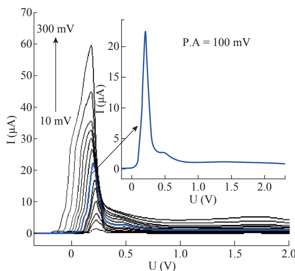
Fig. 9 Wave shapes of 5-FU drug at different pulse time at 10 \mu M, pH = 7 and T = 37 ^{\circ} C.
