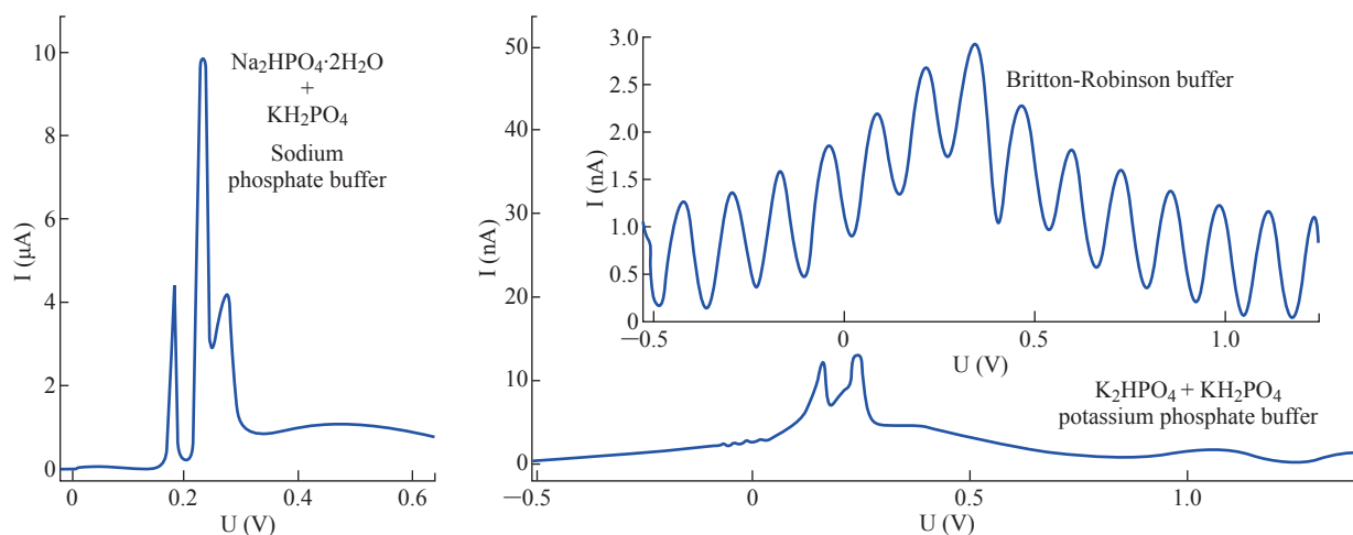
Fig. 4 Polarograms of supporting electrolytes at pH = 7.0 and T = 37 °C by DPP at HMDE.
