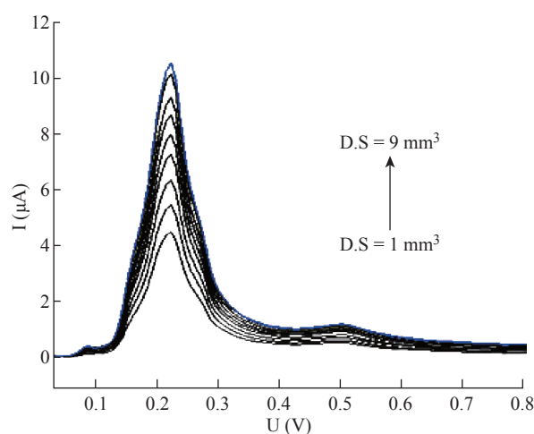
Fig. 6 The mercury drop size in DPP by HMDE of 5-FU drug at 10 \mu M, pH = 7.0 and T = 37 °C.
