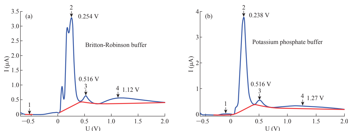
Fig. 5 Polarograms of 5-FU drug (10 \mu M) (a) Britton-Robinson buffer solution, and (b) potassium phosphate buffer solution, at pH = 7.0 and T = 37 °C.
