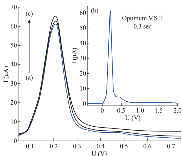
Fig. 11 Polarographic waves of 5-FU (10 \mu\text{M} ) at different V.S.T (a) 0.2, (b) 0.3, (c) 0.03 sec.
