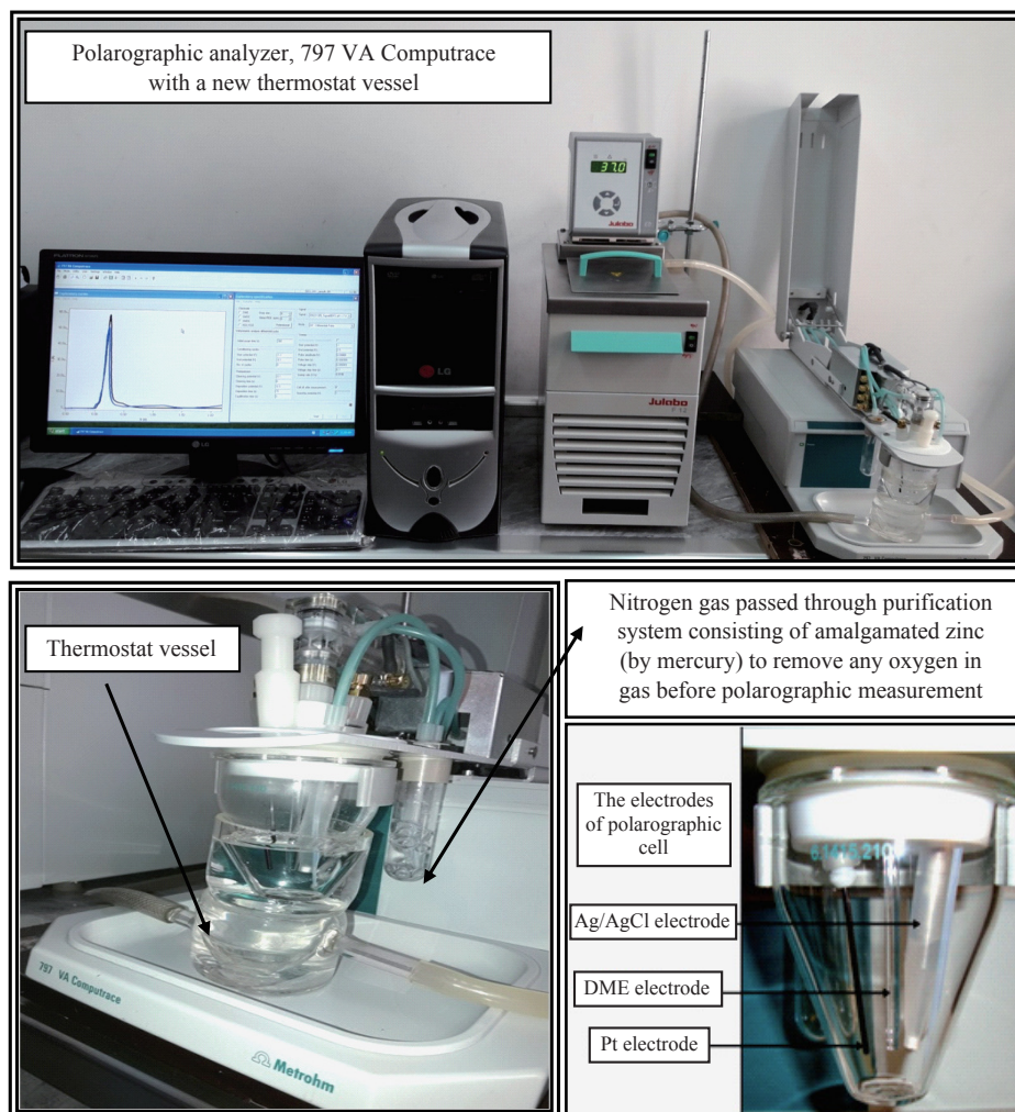
Fig. 2 The new thermostat vessel with a polarographic analyzer, 797 VA Computrace.
