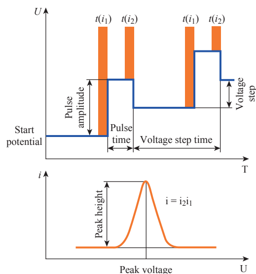
Fig. 7 Differential pulse polarogram and effective sweep parameters [11, 12].
