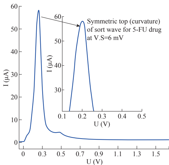
Fig. 10 Polarographic wave of 5-FU (10 \mu\text{M} ) at voltage step = 6 mV in pH = 7 and T = 37 ^{\circ}\text{C} .
