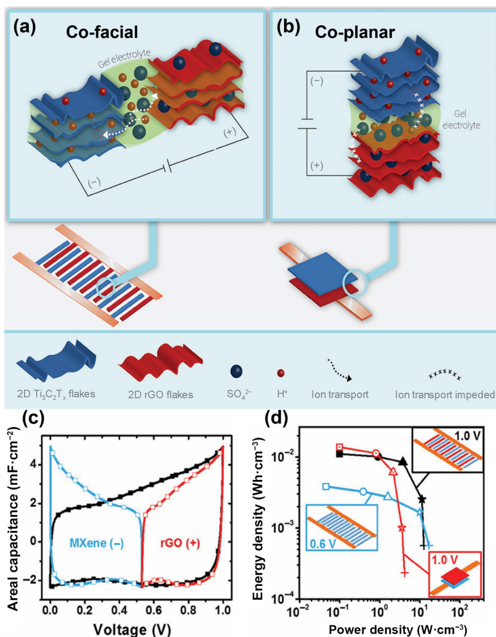
Figure 6 ((a) and (b)) Schematic illustrations of asymmetric FTSCs, (c) CVs of the MSC and the individual electrodes recorded at 2 \text{ mV}\cdot\text{s}^{-1} , and (d) Ragone plot of FTSCs. Reproduced with permission from Ref. [61], © WILEY-VCH Verlag GmbH & Co. KGaA, Weinheim 2017.
