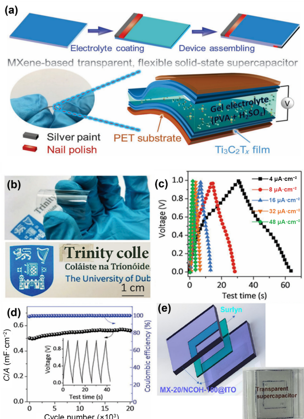
Figure 7 (a) Schematic representation of \text{Ti}_3\text{C}_2\text{T}_x MXene-based FTSC fabrication. (b) Digital images of FTSC, (c) GCD, and (d) durability of the asymmetric FTSC device the asymmetric device. Reproduced with permission from Ref. [62], © WILEY-VCH Verlag GmbH & Co. KGaA, Weinheim 2017. (e) Pictorial representation of MX-20/NCOH-100@ITO symmetric device. Reproduced with permission from Ref. [59], © Elsevier B.V. 2024.
