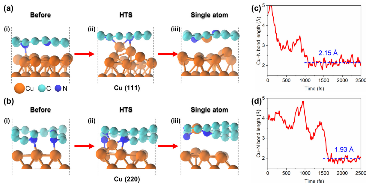
Figure 5 AIMD simulation analysis. (a) Side view of N-C/Cu (111) structure before/during/after HTS. (b) Side view of N-C/Cu (220) structure before/during/after HTS. (c) The bond length evolution of Cu-N in NG/Cu (111). (d) The bond length evolution of Cu-N in NG/Cu (220) during the AIMD simulation at 1300 K within 2.5 ps.
