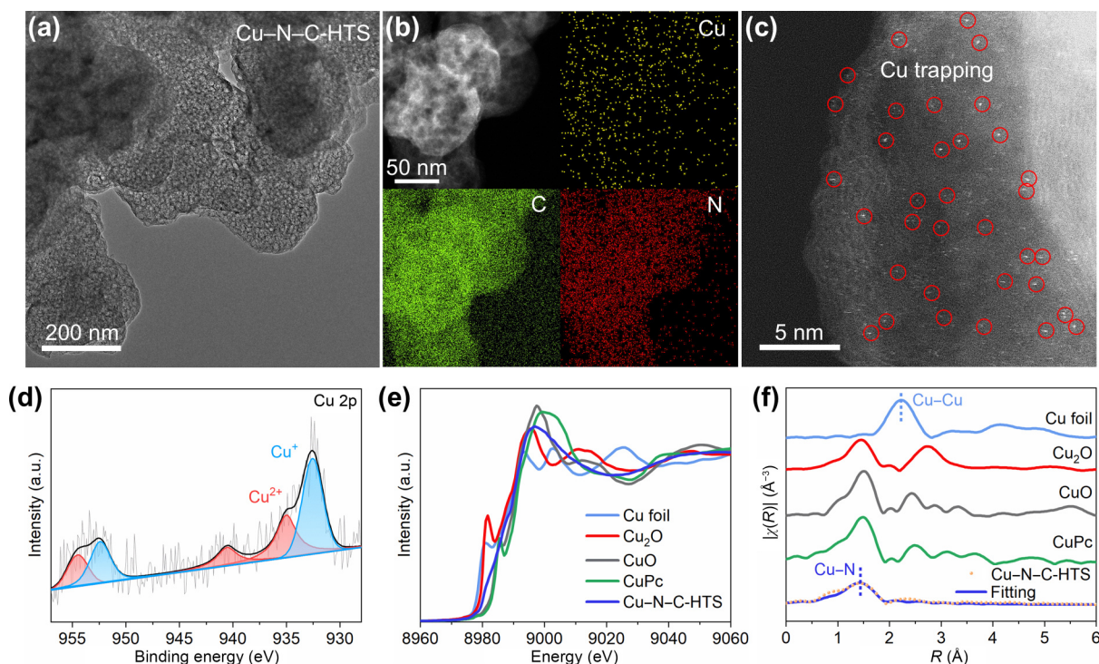
Figure 3 The structural information of Cu-N-C-HTS catalyst. (a) TEM image. (b) STEM image and corresponding elemental mapping, including Cu/C/N. (c) HAADF-STEM image. (d) High-resolution Cu 2p XPS spectrum. (e) Cu K-edge XANES spectra of Cu-N-C-HTS and standard samples of Cu foil, Cu 2 O, CuO, and CuPc. (f) k^2 -weighted ( k ) function of EXAFS spectra and the corresponding fitting curve.
