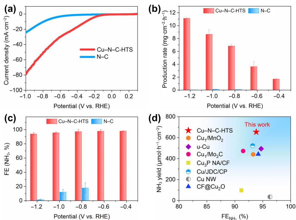
Figure 6 Ammonia synthesis from electrochemical nitrite reduction in 0.1 M KOH and 0.1 M NaNO 2 electrolytes. (a) The LSV polarization curves of N-C and Cu-N-C-HTS catalysts. (b) and (c) Production rate (b) and FE (c) of ammonia over Cu-N-C-HTS and N-C catalysts at different potentials. (d) NO 2 RR performance comparison between Cu-N-C-HTS and recently reported Cu-based catalysts [60–66].
