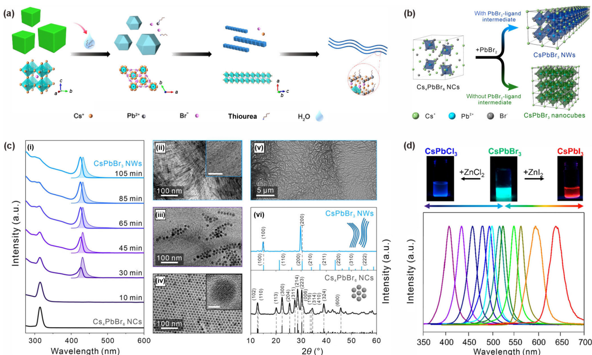
Figure 3 (a) Schematic illustration of the evolution from CsPbBr 3 nanocubes to ultrathin NWs induced by post-synthetic addition of thiourea aqueous solution. Reproduced with permission from Ref. [73], © American Chemical Society 2018. (b) Schematic diagram illustrating the conversion from 0D Cs 4 PbBr 6 perovskite NCs to either ultrathin CsPbBr 3 NWs or CsPbBr 3 nanocubes through selective reaction pathways. (c) Evolution of structure, morphology, and optical properties during the reaction illustrated by: (i) optical absorption and PL spectra depicting the transition from Cs 4 PbBr 6 NCs to ultrathin CsPbBr 3 NWs over time; Corresponding TEM images showing the evolution from (iv) Cs 4 PbBr 6 NCs to (iii) a mixture of Cs 4 PbBr 6 NCs and newly formed CsPbBr 3 NWs, and then (ii) ultrathin CsPbBr 3 NWs; (v) Low-magnification TEM image of NW bundles; (vi) X-ray diffraction (XRD) patterns of starting material and final product. Reproduced with permission from Ref. [75], © American Chemical Society 2021. (d) Photographs of ultrathin CsPbX 3 (X = Cl, Br, I) NW solutions produced via anion exchange (top) and their respective normalized PL spectra (bottom). Reproduced with permission from Ref. [60], © American Chemical Society 2019.
