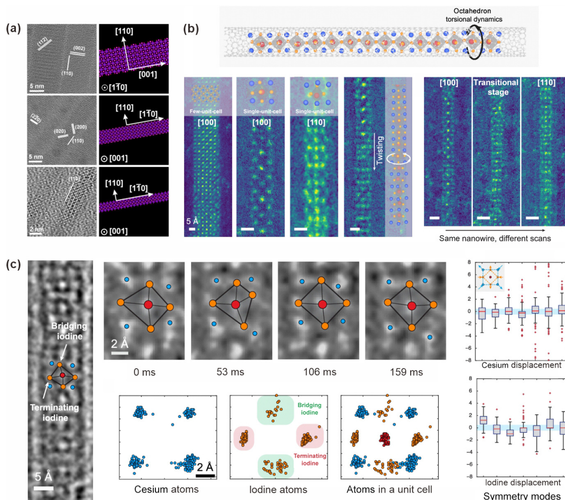
Figure 6 (a) Wide field of view (FOV) HR-TEM images and schematic crystallographic models of synthesized CsPbBr 3 NWs with widths of 10 nm (top row), 5.1 nm (middle row) and 3.4 nm (bottom row). Reproduced with permission from Ref. [47], © American Chemical Society 2016. (b) Schematic model of 1D Cs-Pb-I NWs confined in single-walled carbon nanotubes (top). ADF-STEM characterization of the static structure of atomically thin 1D Cs-Pb-I NWs, viewed along [100], [110], [011] directions, and structural change of the same NW during different scans. (c) Transient structural distortion of individual Pb-I octahedral units, illustrated by atomic-resolution TEM images of Cs-Pb-I NW segments, real-time trajectories of cesium (blue), lead (red) and iodine (orange) atoms, and unit-cell framework distortion of cesium and iodine decomposed based on seven symmetry modes of a square. Reproduced with permission from Ref. [87], © American Chemical Society 2023.
