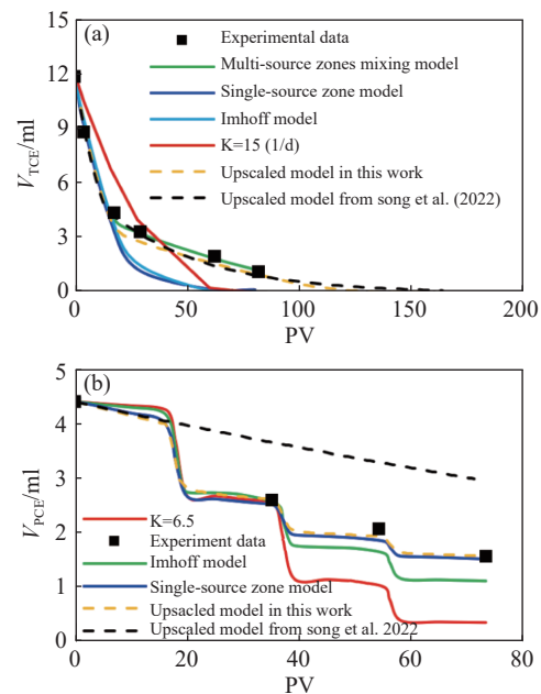
Fig. 4 The remaining DNAPL volume ( V ) in the flow cell varying with the pore volume of injected flushing fluid (PV)
