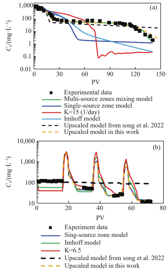
Fig. 3 The simulated elution concentration ( C_2 ) from the upscaled analytical solution model and numerical model, respectively
