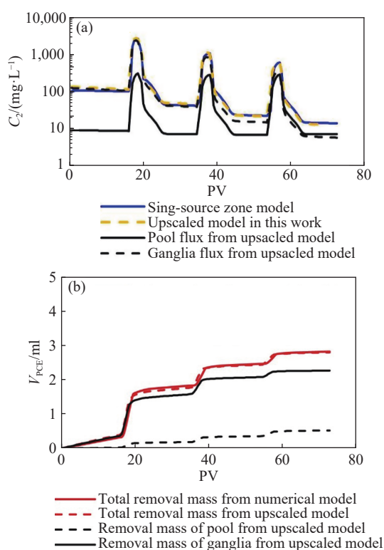
Fig. 11 Contaminant fluxes ( C_2 , a) and removal mass ( V_{PCE} , b) from the pool- and ganglia-dominated DNAPL source regions predicted by the upscaled analytical solution model and the numerical model in Experiment B
