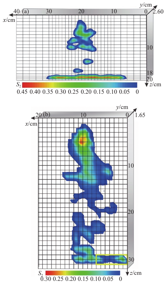
Fig. 2 The initial DNAPL distribution before flushing
