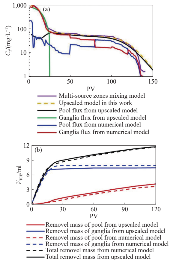
Fig. 10 Contaminant fluxes ( C_2 , a) and removal mass ( V_{TCE} , b) from the pool- and ganglia-dominated DNAPL source regions predicted by the upscaled analytical solution model and the numerical model in Experiment A
