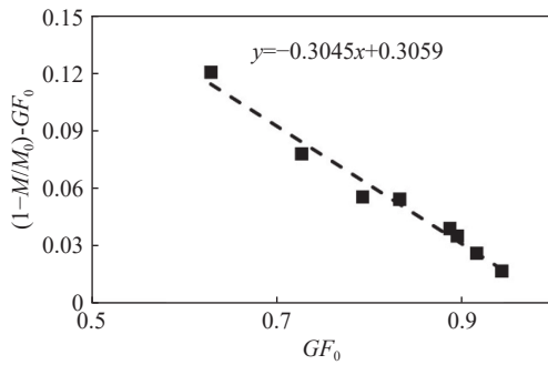
Fig. 7 The relationship between the removal ratio of DNAPL in the contaminated region, i.e. , (1-M/M_0) , and the initial proportion of DNAPL ganglia ( GF_0 ) when the elution curve enters the second stage
