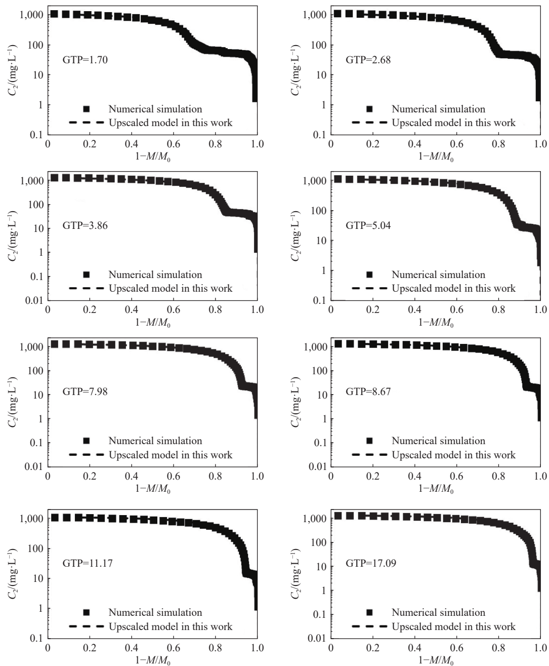
Fig. 6 Under different initial DNAPL distributions (GTP), the prediction of elution concentration ( C_2 ), from the upscaled analytical solution model and the numerical model (multi-source zone mixing model), varying with DNAPL depletion ratio ( 1-M/M_0 )
