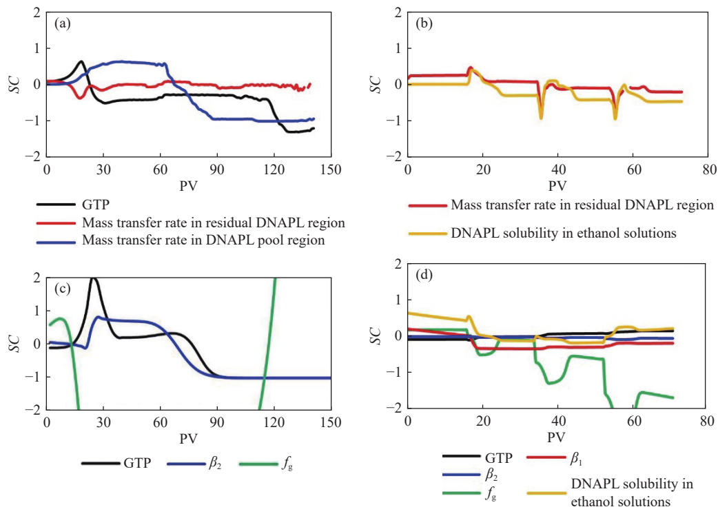
Fig. 9 Sensitivity Coefficients (SC) of key parameters for the numerical model predicting the effluent concentration under
