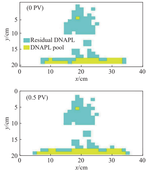
Fig. 1 Comparison of DNAPL distributions at different times (PV) in the mixed-source experiment
