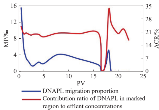
Fig. 5 DNAPL Migration Proportion (MP) and average contribution ratio of DNAPL to effluent concentrations in the marked zone (ACR)
