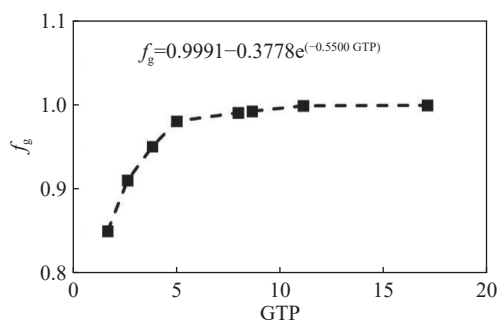
Fig. 8 The relationship between the proportion of the flux from DNAPL ganglia ( f_g ) and the initial DNAPL distribution (GTP)
