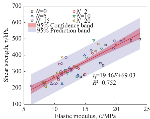
Fig. 7 The relationship curve between the elastic modulus and the shear strength
