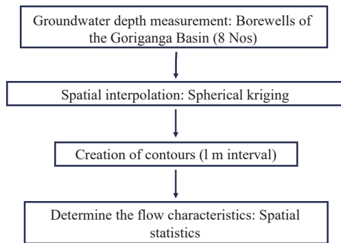
Fig. 4 Flowchart of the methodological framework for studying groundwater flow characteristics (Fig. 5).
