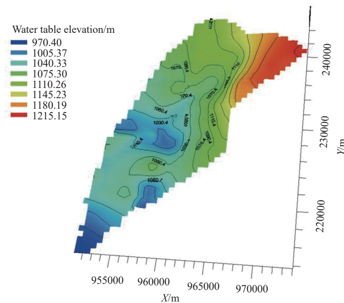
Fig. 12 Reconstitution of the piezometric state in transient regime, June 2021
