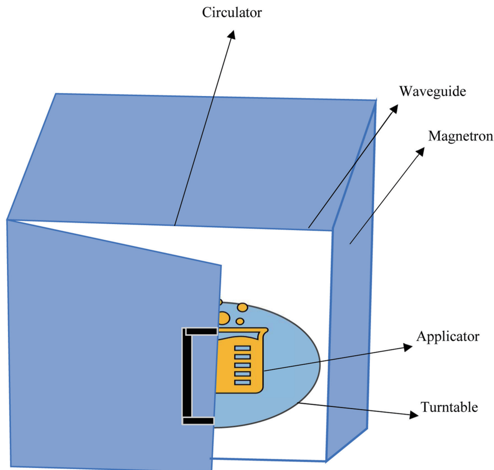
Figure 1. Microwave instrumentation.
