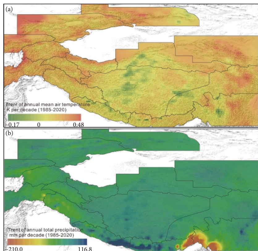
Fig. 2 Changes in annual average temperature and multi-year average total precipitation in HMA from 1985 to 2020, based on ERA5 reanalysis data. (a) Change in annual average temperature from 1985 to 2020. (b) Change in multi-year average total precipitation from 1985 to 2020. The black solid line indicates the boundary of the Global Terrestrial Network for Glaciers (GTN-G) regions.
