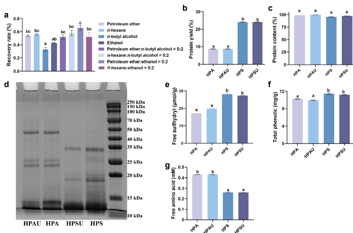
Figure 1 (a) Hemp seeds powder recovery for different oil extraction methods; (b) protein yields for different extraction methods; (c) protein purity measurement; (d) electropherograms of the four types of protein extracts; (e) free sulphydryl content ( \mu\text{mol/g} ); (f) total phenolic content (mg/g); (g) free amino content (mmol/L).
