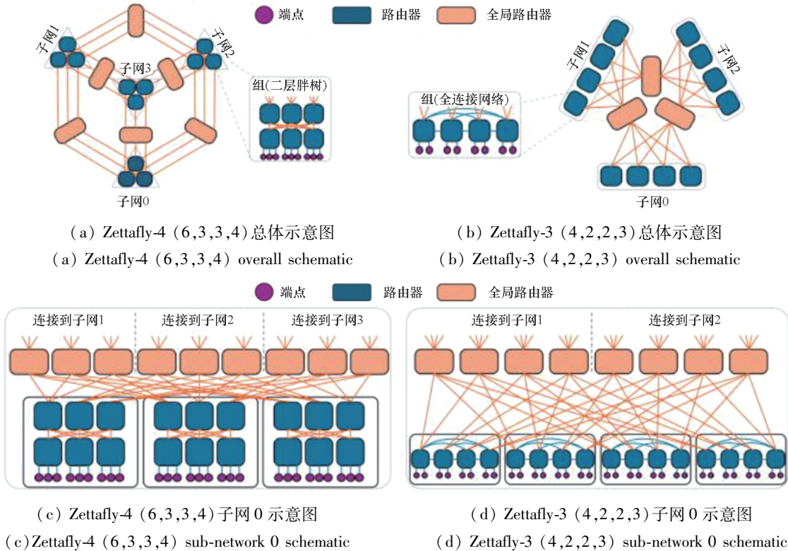
图 14 Zettafly-3 (4,2,2,3) 和 Zettafly-4 (6,3,3,4) 网络 Fig. 14 Zettafly-3 (4,2,2,3) and Zettafly-4 (6,3,3,4) networks
