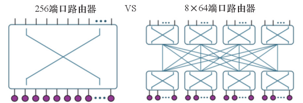
图 17 “大芯片小网络”和“小芯片大网络”的权衡 Fig. 17 Trade off between chip throughput and network size
