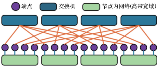
图 10 两层 Rail-Only 网络 Fig. 10 Two-layer Rail-Only network
