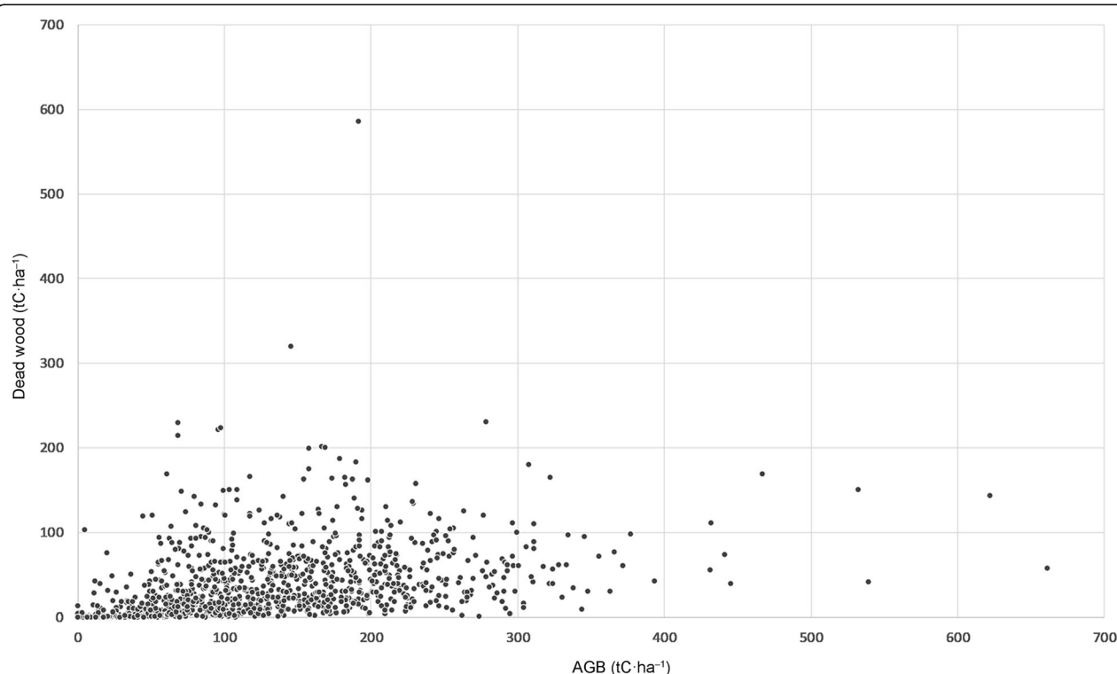
Fig. 2 Remeasurement plots in tall forests ( n = 803 ) showing dead wood carbon stocks ( \text{tC}\cdot\text{ha}^{-1} ) plotted against total AGB carbon stocks ( \text{tC}\cdot\text{ha}^{-1} ). Data are from the first measurement cycle 2002–2007
