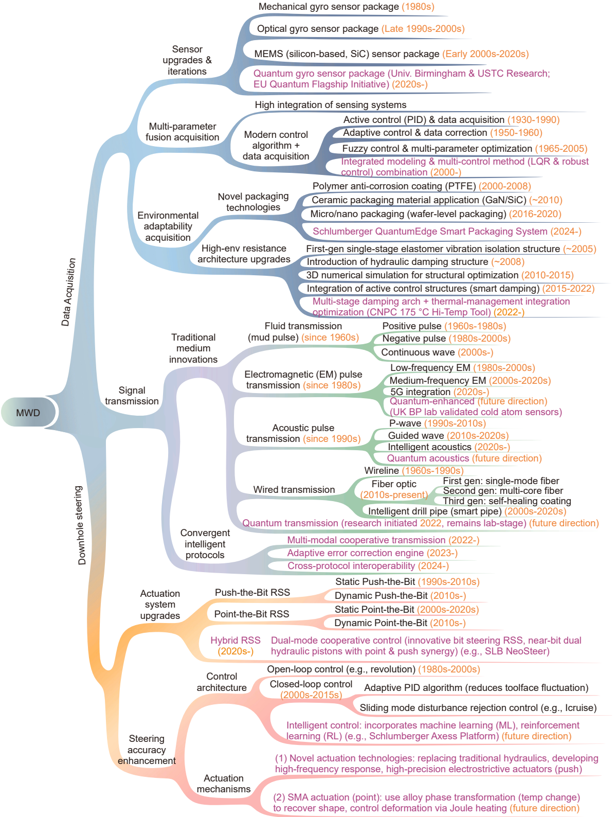
Fig. 13. Hierarchical trend analysis of MWD “acquisition-transmission-drilling” workflow.
