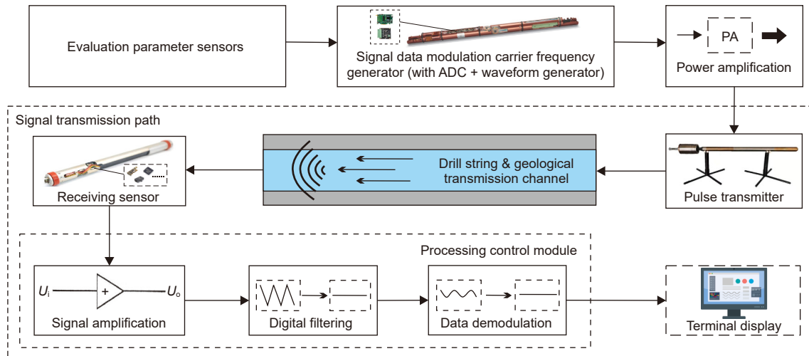
Fig. 7. MWD signal transmission flow (one-way scheme).
