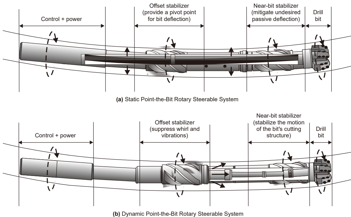
Fig. 11. Schematic diagram of Point-the-Bit Rotary Steerable System action.
