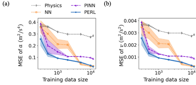
Fig. 11. PERL (LSTM + IDM) and baseline prediction performance: (a) acceleration prediction result and (b) speed prediction result.
