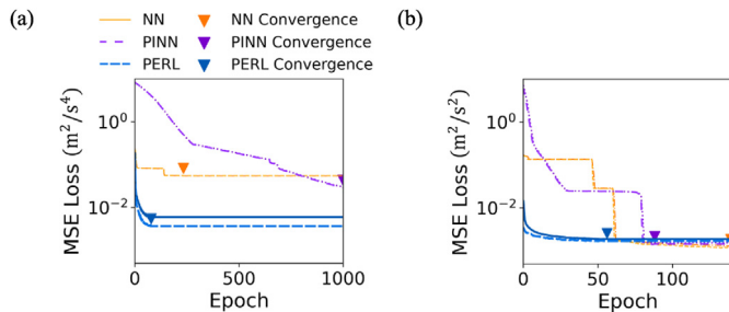
Fig. 14. Training processes of PERL (LSTM + FVD) and baseline models: (a) training data size = 500 and (b) training data size = 1,500.
