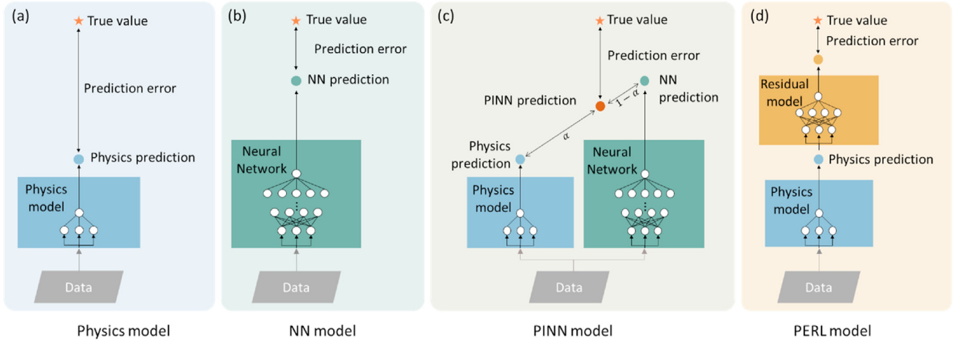
Fig. 1. General structure of the PERL model and three existing models: the physics model, NN model, and PINN model.
