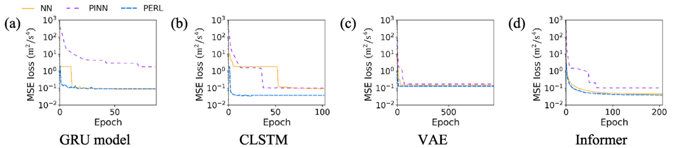
Fig. 10. Training processes of the NN, PINN, and PERL structure using various models with a sample size of 15,000, utilizing various learning-based models: (a) GRU model, (b) CLSTM model, (c) VAE model, and (d) Informer model.
