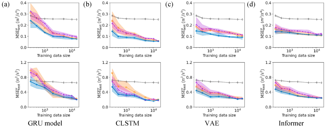
Fig. 5. PERL and baseline prediction performance of different learning-based models.
