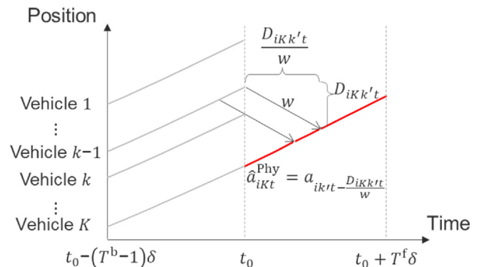
Fig. 3. Adapted Newell model for vehicle trajectory prediction.
