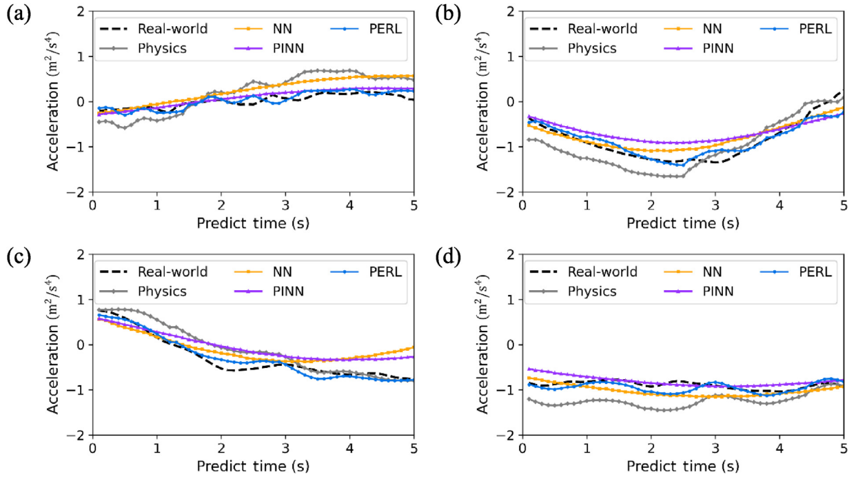
Fig. 8. Comparison of real-world acceleration and predicted results of the PERL (Newell + CLSTM) model and baseline models under four different driving scenario: (a) acceleration, (b) deceleration, (c) cruise, and (d) deceleration.
