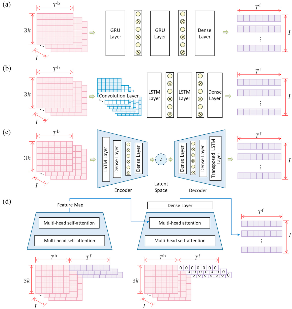
Fig. 4. Model structures of (a) GRU model, (b) CLSTM model, (c) VAE model, and (d) Informer model.
