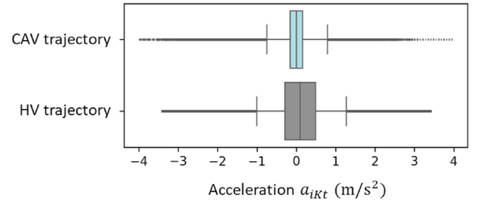
Fig. 15. Comparison of the acceleration distributions in the CAV and HV trajectory datasets.
