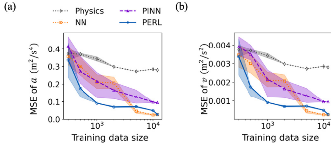
Fig. 13. PERL (LSTM + IDM) and baseline prediction performance: (a) acceleration prediction result and (b) speed prediction result.
