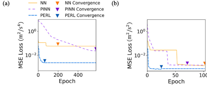
Fig. 12. Training processes of PERL (LSTM + IDM) and baseline models: (a) training data size = 500 and (b) training data size = 1,500.
