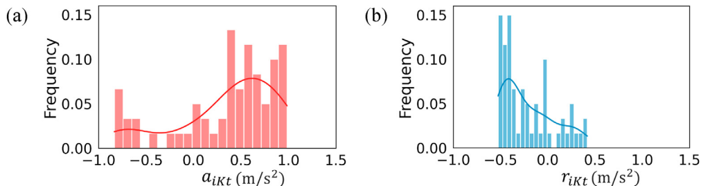
Fig. 7. Differences in the distributions of (a) acceleration a_{ikt} and (b) acceleration residual r_{ikt} in one sample.
