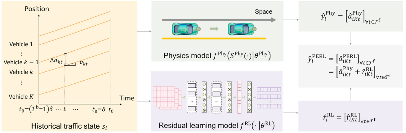
Fig. 2. Workflow of the PERL model (examples of vehicle trajectory prediction).
