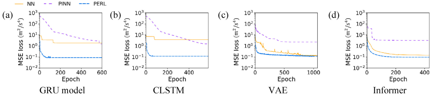
Fig. 9. Training processes of the NN, PINN, and PERL structure using various models with a sample size of 1,000, utilizing various learning-based models: (a) GRU model, (b) CLSTM model, (c) VAE model, and (d) Informer model.
