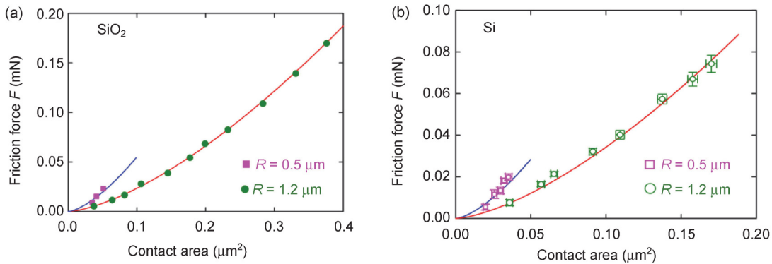
Fig. 13 Friction force as a function of contact area. Only the data in the elastic region are shown.
