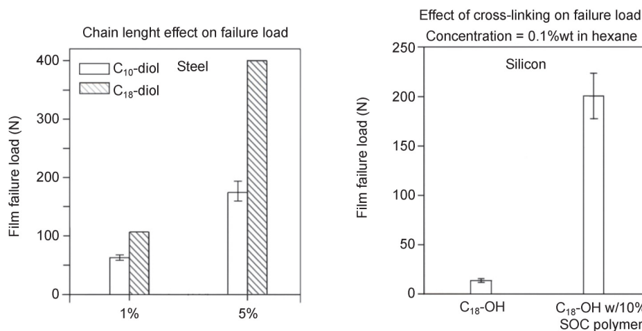
Fig. 25 Effect of chain-length and cross-linking on failure load.
