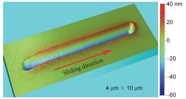
Fig. 11 AFM image of a groove created on \text{CaF}_2 .
