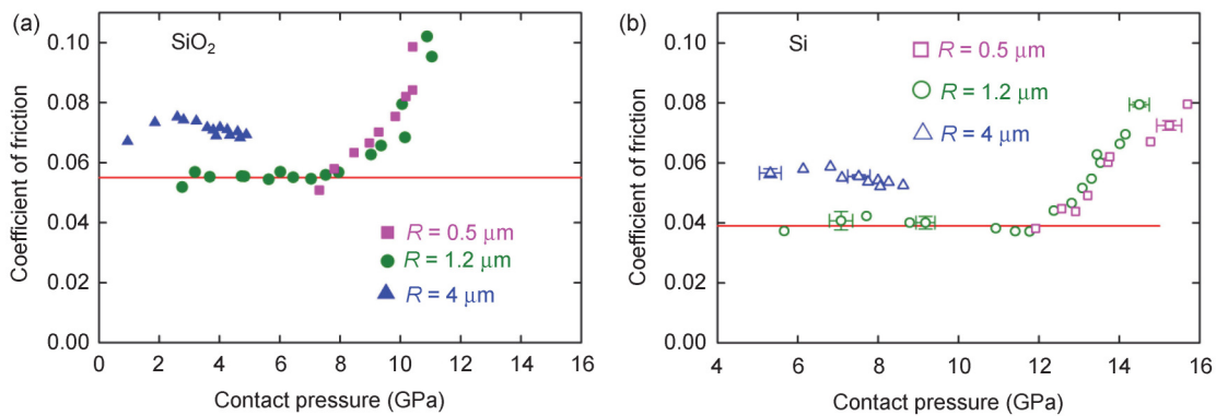
Fig. 9 Coefficient of friction as a function of contact pressure.
