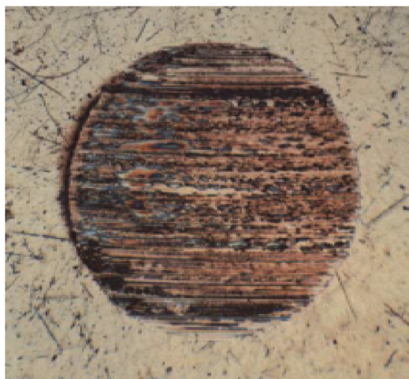
Fig. 19 A lubricated wear scar in a four ball wear test conducted under ZDDP added paraffin oil at 40 kg, 600 rpm, and 25 °C, after one minute of sliding. The wear scar diameter is 0.55 mm.
