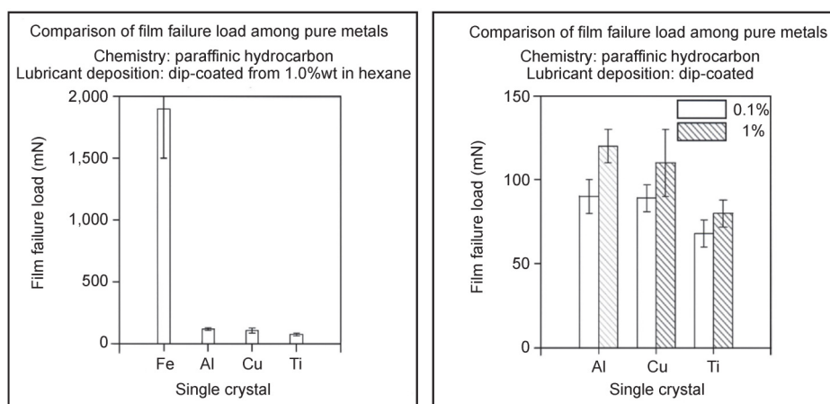
Fig. 24 Comparison of film rupture load among pure metals.
