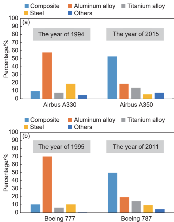
图1 民用飞机重点机型机身各类材料占机体结构总量变化 [7] (a)空客公司;(b)波音公司 Fig. 1 Changes in amount of different types of materials in total base structure in fuselage of key civil aircraft models [7] (a)Airbus; (b)Boeing
