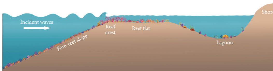
Fig. 1 A typical coral reef profile.
