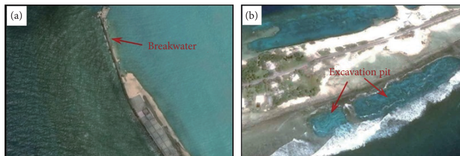
Fig. 5 (a) Breakwaters on a reef flat at Yongxing island in the South China Sea; (b) Excavation pit at Majuro Atoll in the Republic of the Marshall Islands (images from Google Map).
